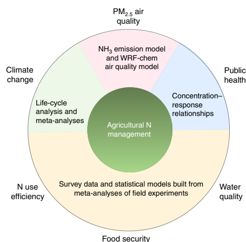
Fig. 1 | An integrated assessment framework for evaluating the impacts of improved N management in China. Impacts on PM_{2.5} were evaluated using the NH_3 emission model from Zhang et al. 26 and the WRF-Chem air quality model. Concentration-response relationships for impacts of fine particulates on premature mortality were analysed using methods from Burnet et al. 31 . Other impacts were estimated using life-cycle GHG analysis (as in Zhang et al. 51 ), statistical models of N application rates and Nr emissions, farm surveys of crop yields and N use, and several meta-analyses of field experiments that evaluate impacts of N management on Nr emissions and yields 79,18,70,71 .
